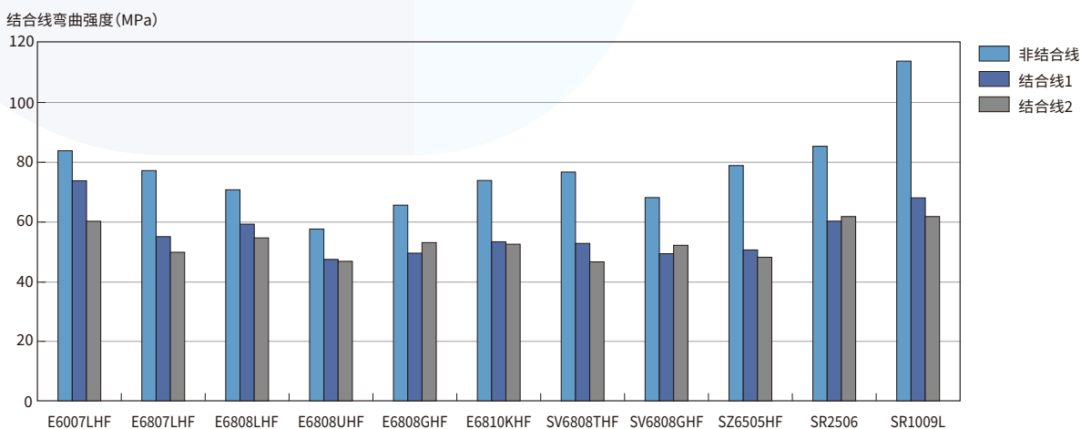
图3-2-9 SUMIKASUPER LCP 结合线弯曲强度(0.5mm 厚度)
