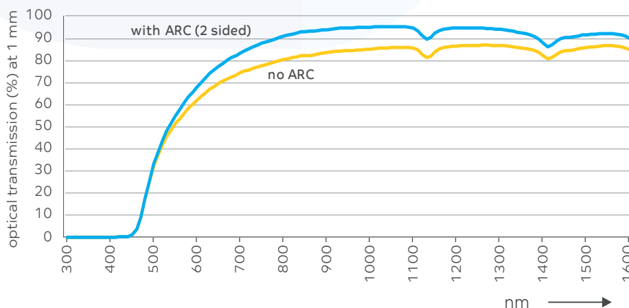
EXTEM™ RH1016UCL RESIN OPTICAL TRANSMISSION IMPROVEMENT USING ANTI REFLECTIVE COATING (ARC)
