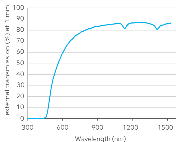
EXTERNAL TRANSMISSION OF EXTEM RH1016UCL RESIN
