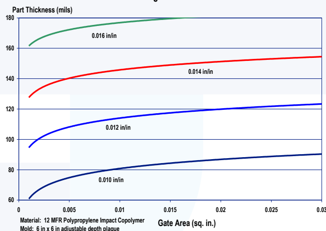
Contour Plots of Constant Mold Shrinkage as a Function of Gate Area and Part Thickness
