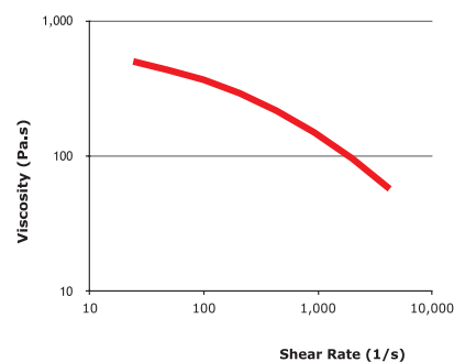
Shear-Viscosity @ 190 °C
