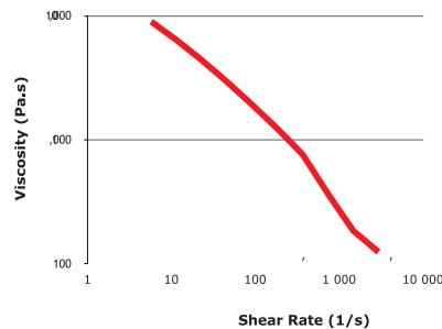
Shear-Viscosity @ 190 °C
