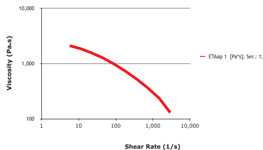
Shear-Viscosity @ 190 °C
