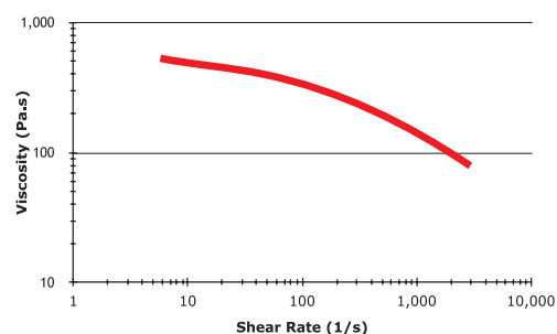
Shear-Viscosity @ 190 °C
